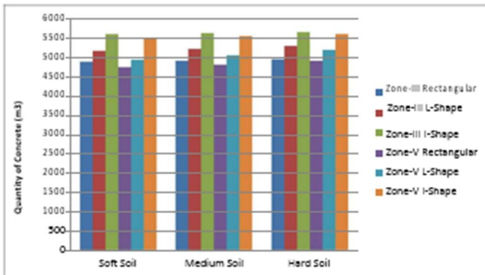
Fig:3 quantity of concrete (cum)
