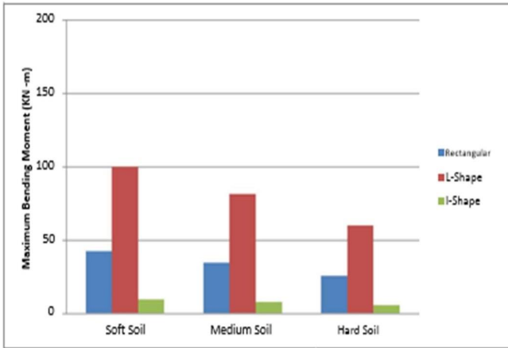
Fig:2 Maximum bending moment.
