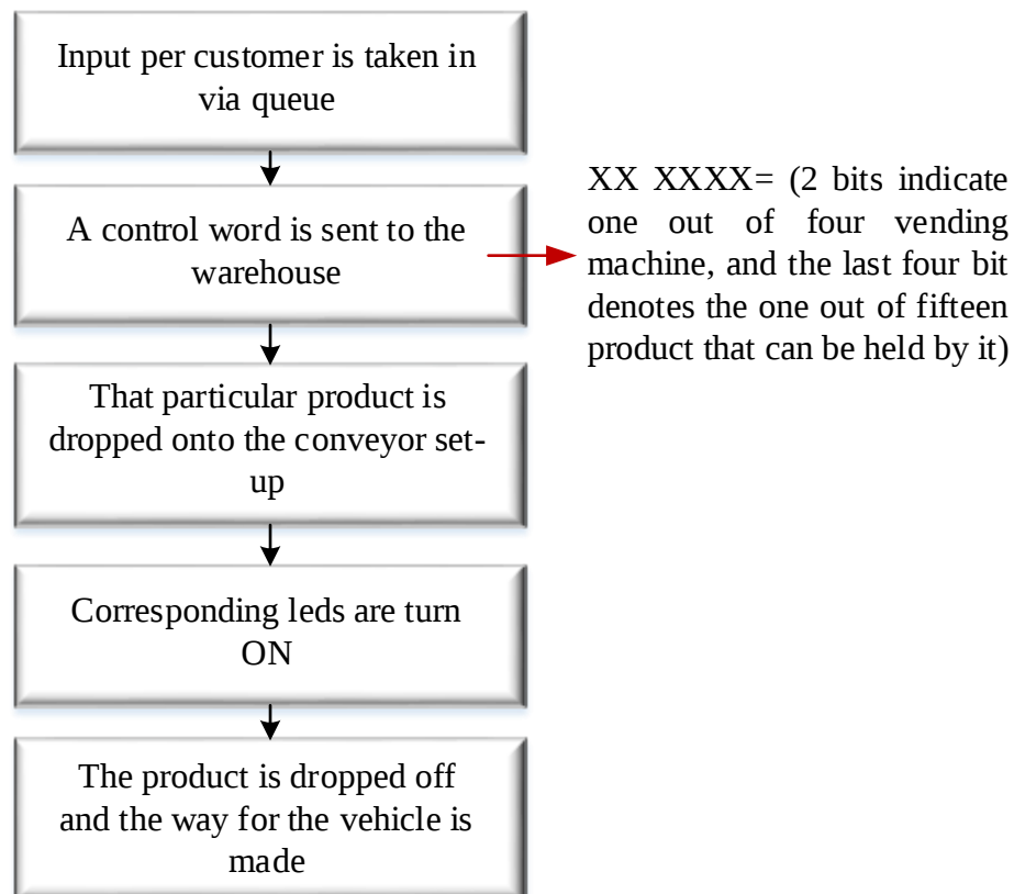
Fig 4: Flow chart of our proposed method
