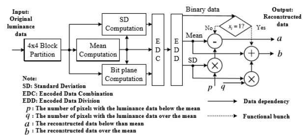
Figure 1: Block diagram of Block Truncation Coding
