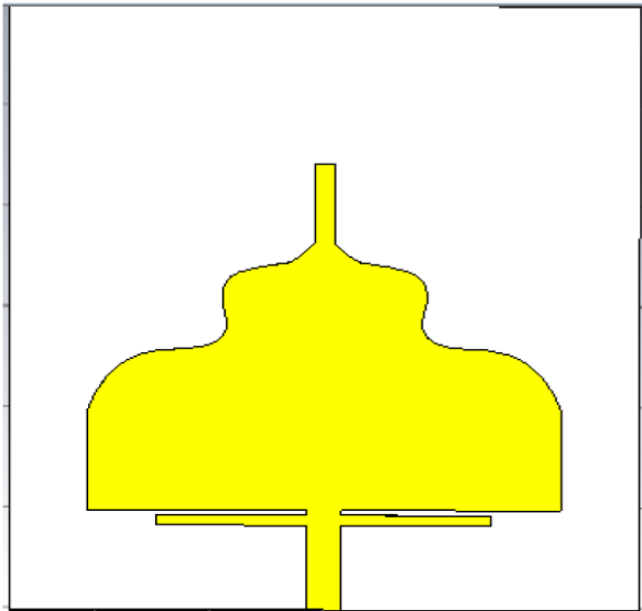
Figure 3: Parasol Design of Microstrip Antenna
