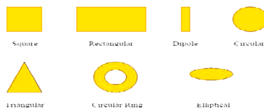
Figure 2: Common shapes of microstrip patch element
