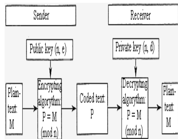
Fig 1. RSA algorithm
