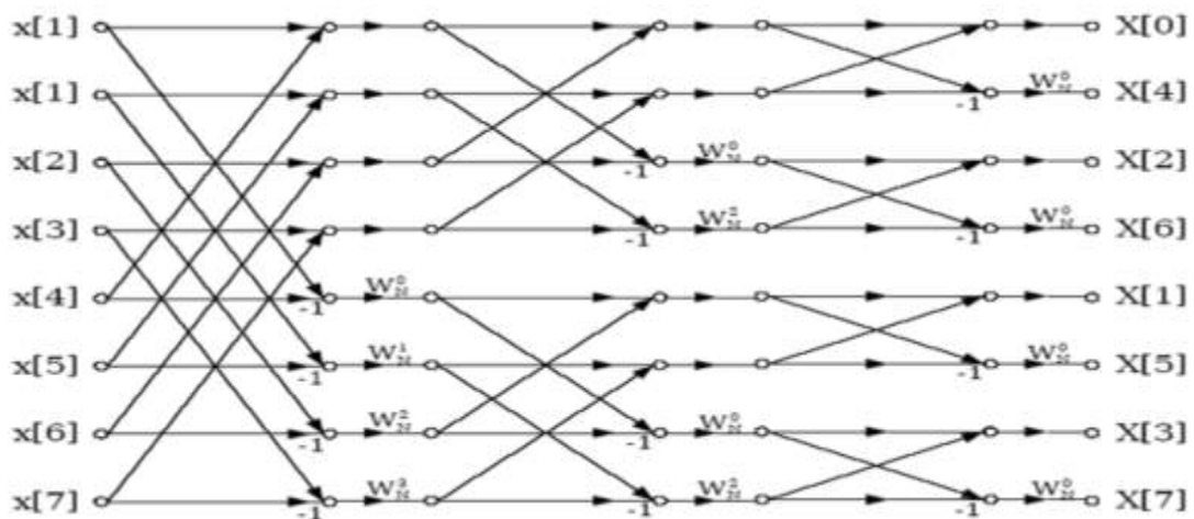
Figure 2: 8-point DIF-FFT Radix-2 Butterfly
