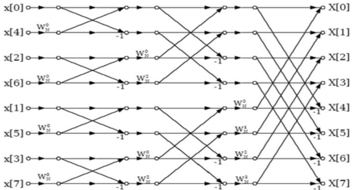
Figure 1: 8-point DIT-FFT Radix-2 Butterfly
