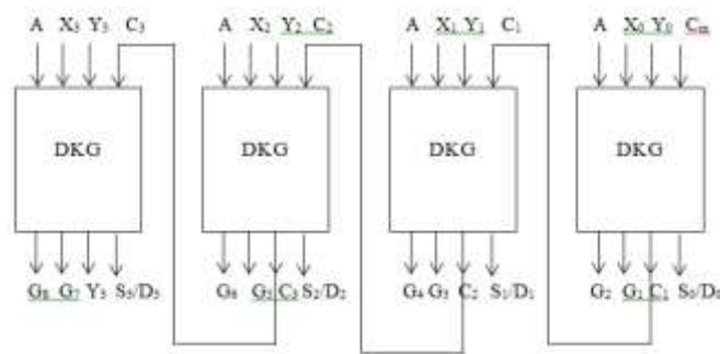
Figure 7: Reversible 4-bit Adder/ Sub tractor using DKG Gate
