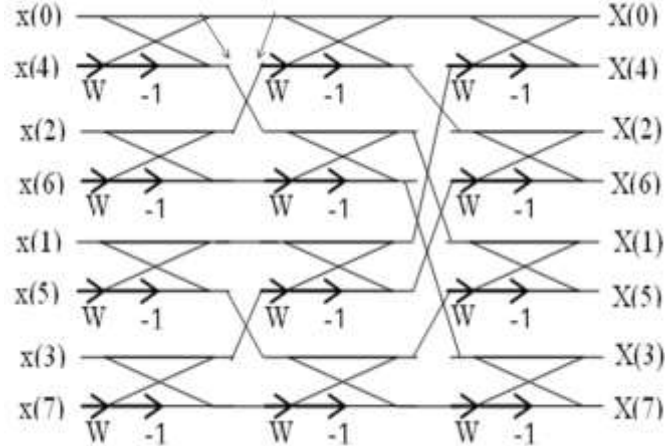
Figure 8: Flow Diagram of FFT using Folding Technique
