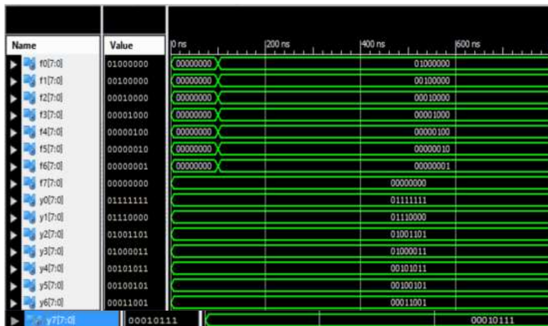
Figure 11: Output Waveform of DIT 8-point FFT using DKG Gate
