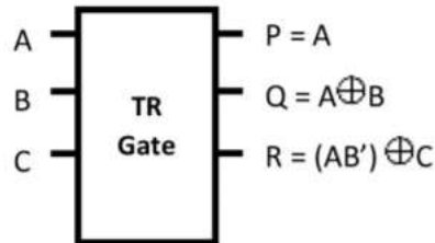
Figure 4: Block Diagram of TRG
