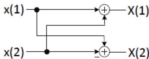
Figure 6: Radix-2 Butterfly
