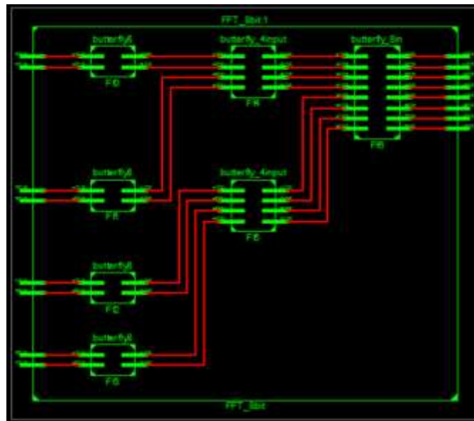
Figure 10: RTL View of DIT 8-point DIT-FFT algorithm
