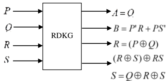
Figure 5: DKG Gate
