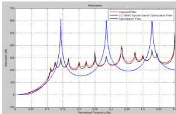
Figure 7: Attenuation Graph of 2 \times 2 MIMO system based Optimization Filter
