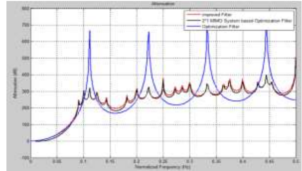
Figure 4: Attenuation Graph of 2×1 MIMO system based Optimization Filter
