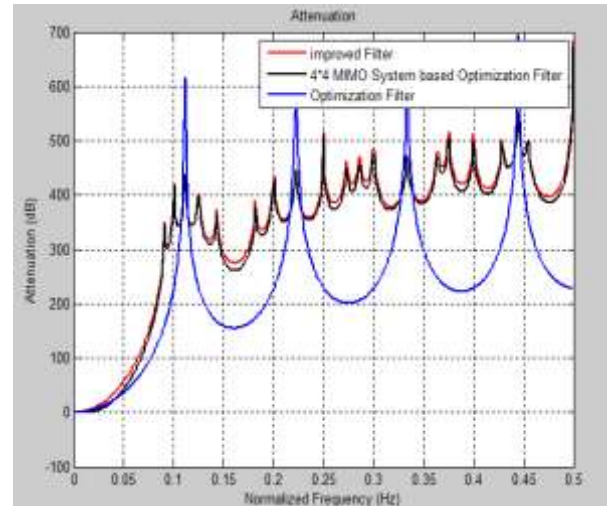
Figure 10: Attenuation Graph of 4 \times 4 MIMO system based Optimization Filter
