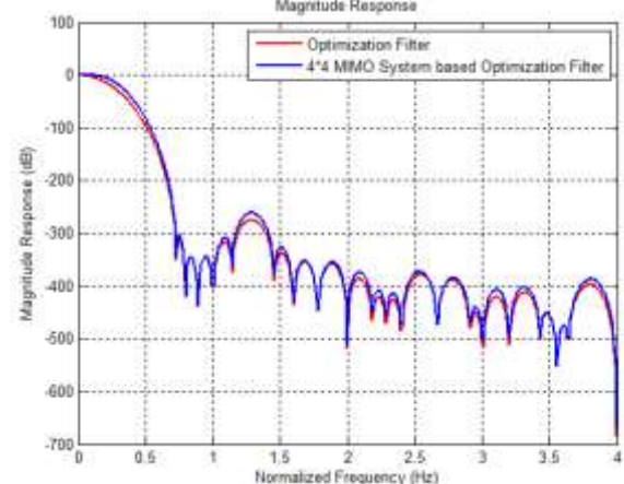
Figure 11: Magnitude Response of 4 \times 4 MIMO system based Optimization Filter
