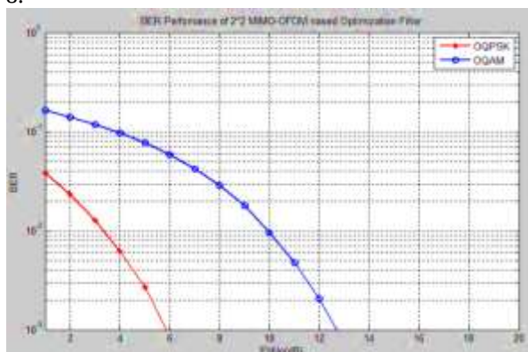
Figure 9: BER Analysis of 2 \times 2 MIMO system based Optimization Filter
