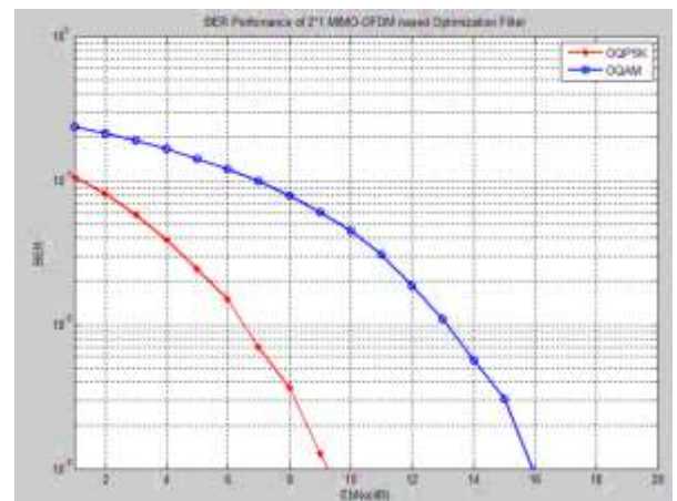
Figure 6: BER Analysis of 2×1 MIMO system based Optimization Filter
