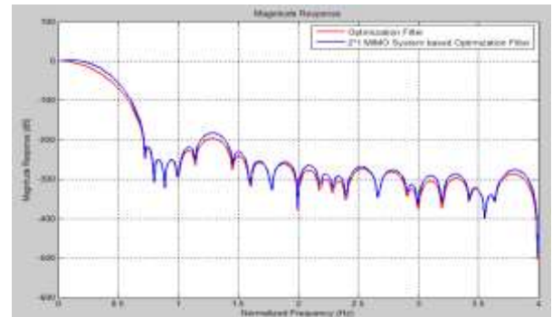
Figure 5: Magnitude Response of 2×1 MIMO system based Optimization Filter
