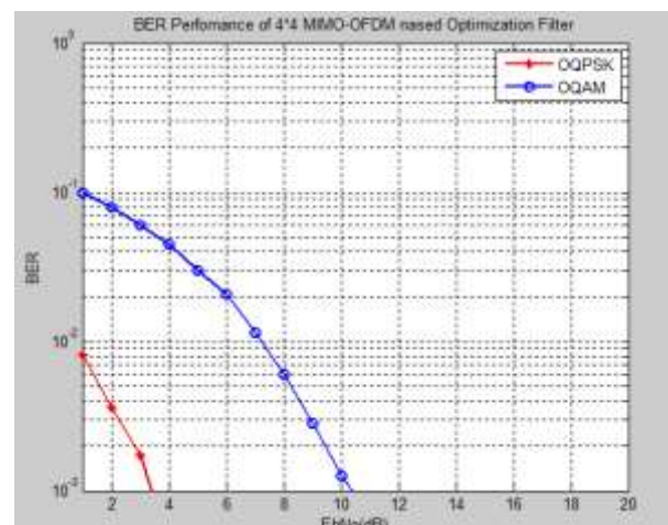
Figure 12: BER Analysis of 4 \times 4 MIMO system based Optimization Filter
