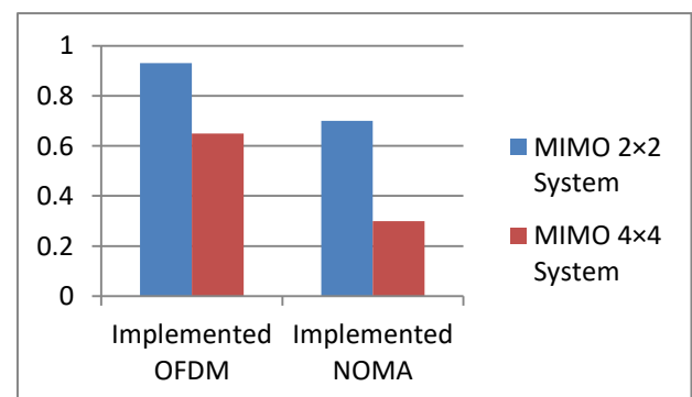
Fig. 12: Comparison BER Result for OFDM Vs NOMA for SNR = 0 dB
