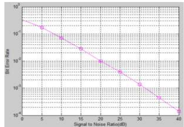
Fig. 11: BER for MIMO 4x4 System
