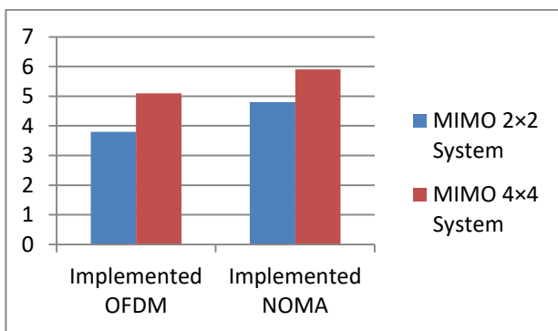
Fig. 14: Comparison Throughput Result for OFDM Vs NOMA for SNR = 0 dB
