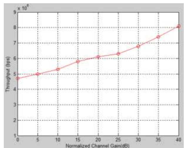
Fig. 7: Throughput for MIMO 2x2 System
