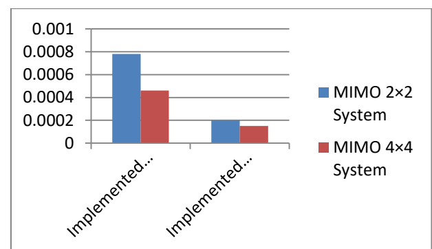
Fig. 13: Comparison BER Result for OFDM Vs NOMA for SNR = 40 dB
