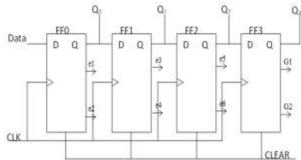
Figure 3: Flow Diagram of Parallel in Serial Output Shift Register
