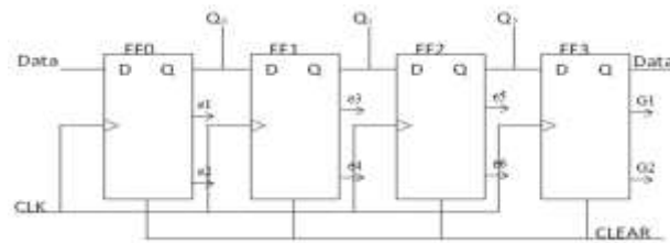
Figure 2: Flow Diagram of Serial in Parallel Output Shift Register
