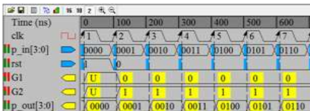
Figure 8: Output Waveform of 4-bit Parallel in Parallel out Shift Register
