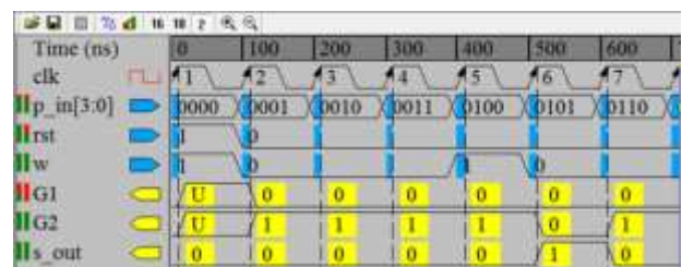
Figure 7: Output Waveform of 4-bit Parallel in Serial out Shift Register
