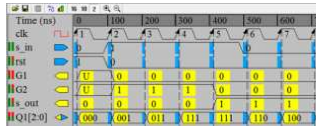
Figure 6: Output Waveform of 4-bit Serial in Serial Out Shift Register
