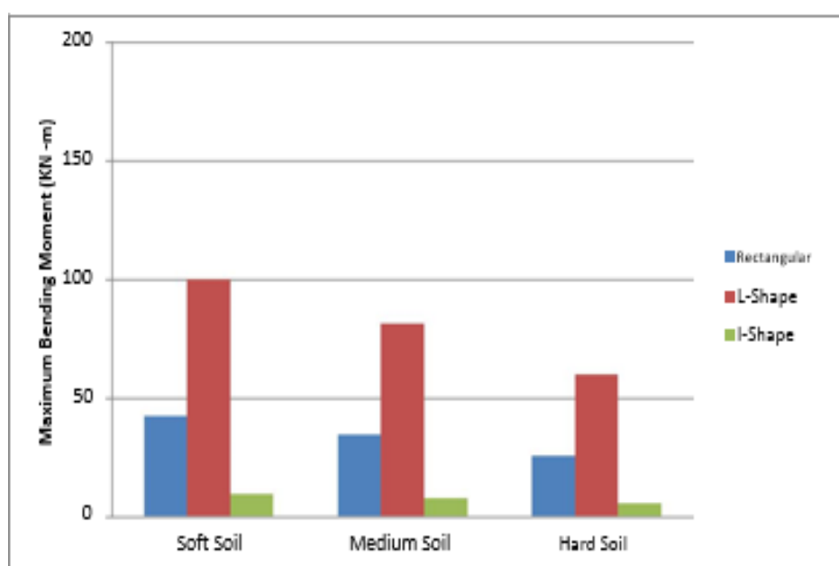
Fig:2 Maximum bending moment.
