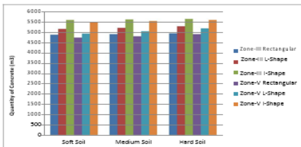
Fig:3 quantity of concrete (cum)
