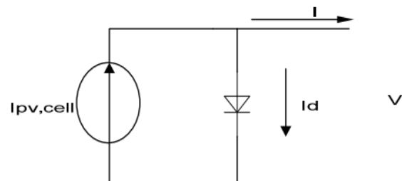
Figure 3: Show ideal photovoltaic cell equivalent circuit
