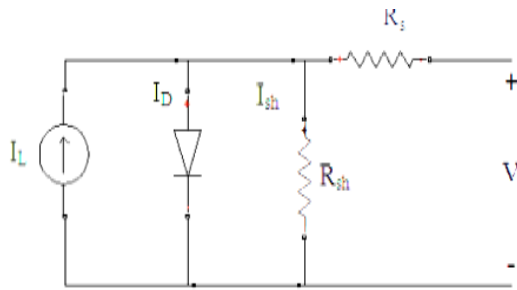
Figure 4: Equivalent Electrical Circuit of PVC
