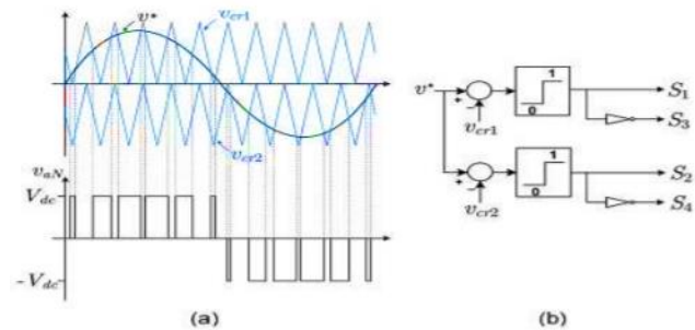
Figure 2: Phase Shift PWM
