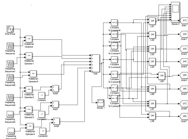
Figure 6: Simulation Model of Proposed Methodology
