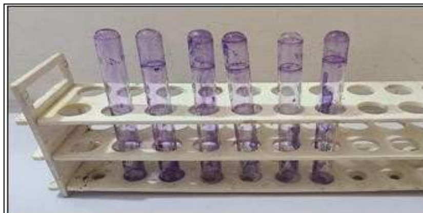
Figure 6: Anti biofilm activity of Polymeric Nanoparticles against Bacillus subtilis
