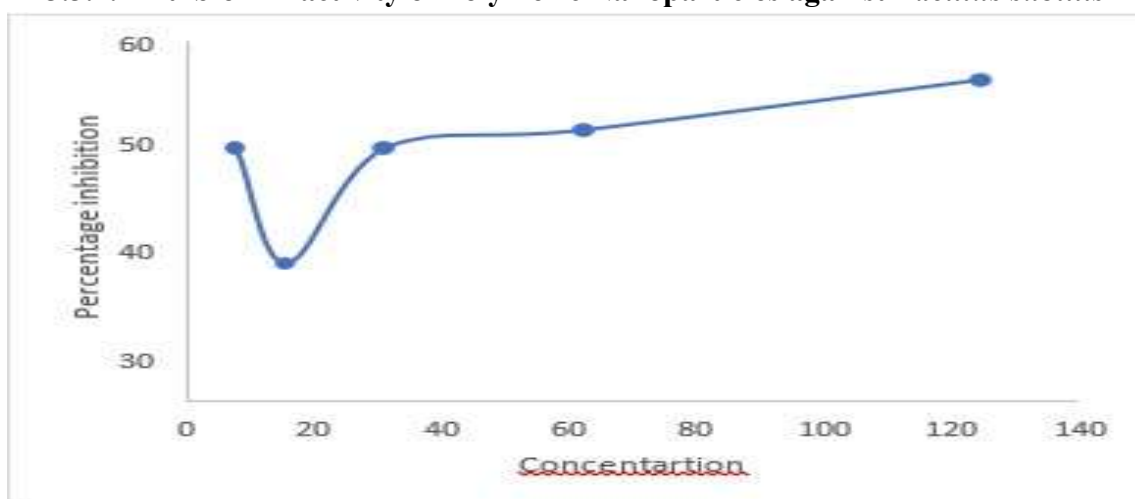
Graph 11: Graph represents anti biofilm activity of Bacillus subtilis
