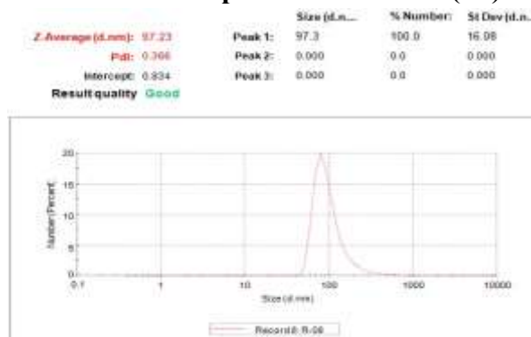
Graph 4: Particle Size (F4)
