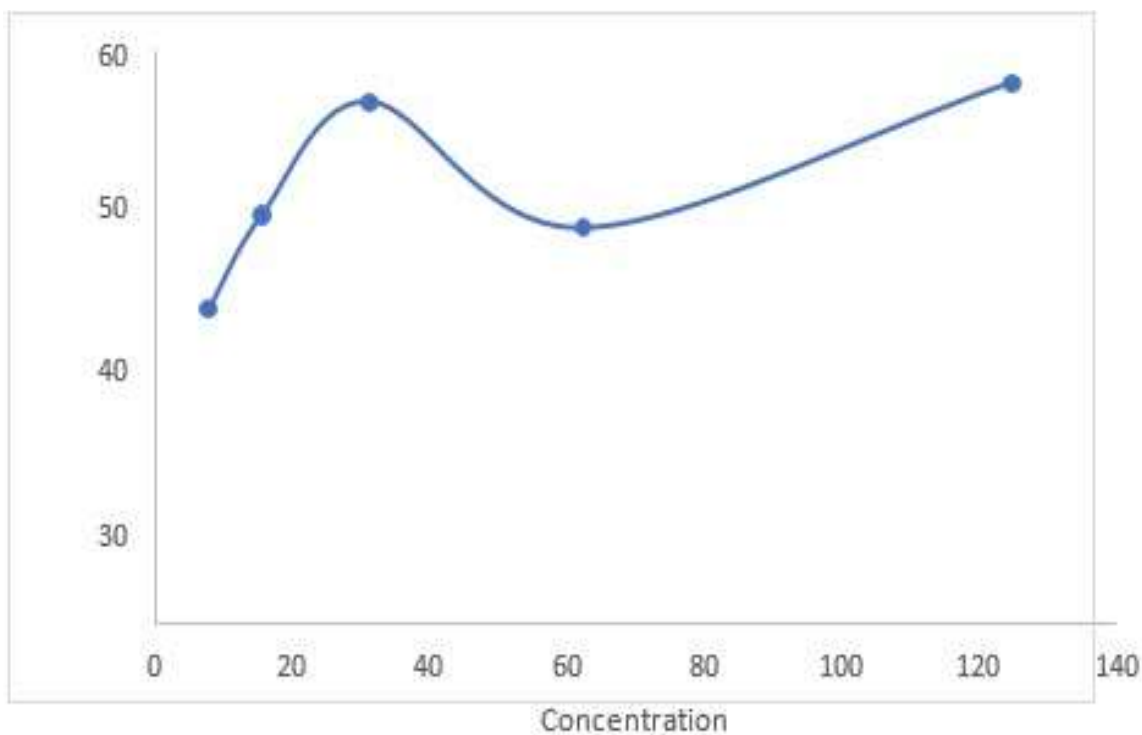
Graph 12: Graph represents anti biofilm activity of Pseudomonas aeruginosa
