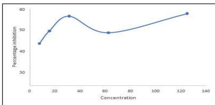
Graph 14: Graph represents anti biofilm activity of Pseudomonas aeruginosa
