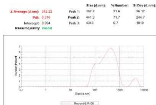
Graph 1: Particle Size (F1)
