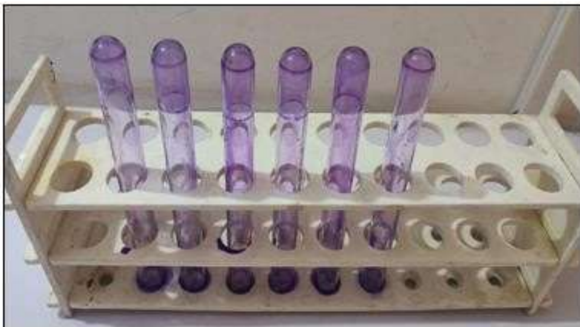
Figure 5: Anti-biofilm activity of Polymeric Nanoparticles against Pseudomonas aeruginosa
