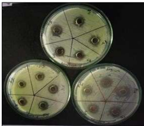
Figure 3: Antibacterial activity of Polymeric Nanoparticles against Pseudomonas aeruginosa
