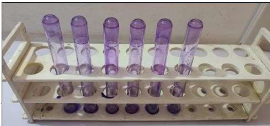
Figure 7: Anti-biofilm activity of Polymeric Nanoparticles against Pseudomonas aeruginosa The anti-biofilm activity of the nanoparticle was assessed using the test tube method. The maximum percentage inhibition of bacterial growth at 125µg/ml highlights the potential effectiveness of a compound or formulation against two significant pathogens. exhibited a Bacillus subtilis and Pseudomonas aeruginosa remarkable inhibition rate 53.47% and 56.57% and showed a zone of inhibition.
