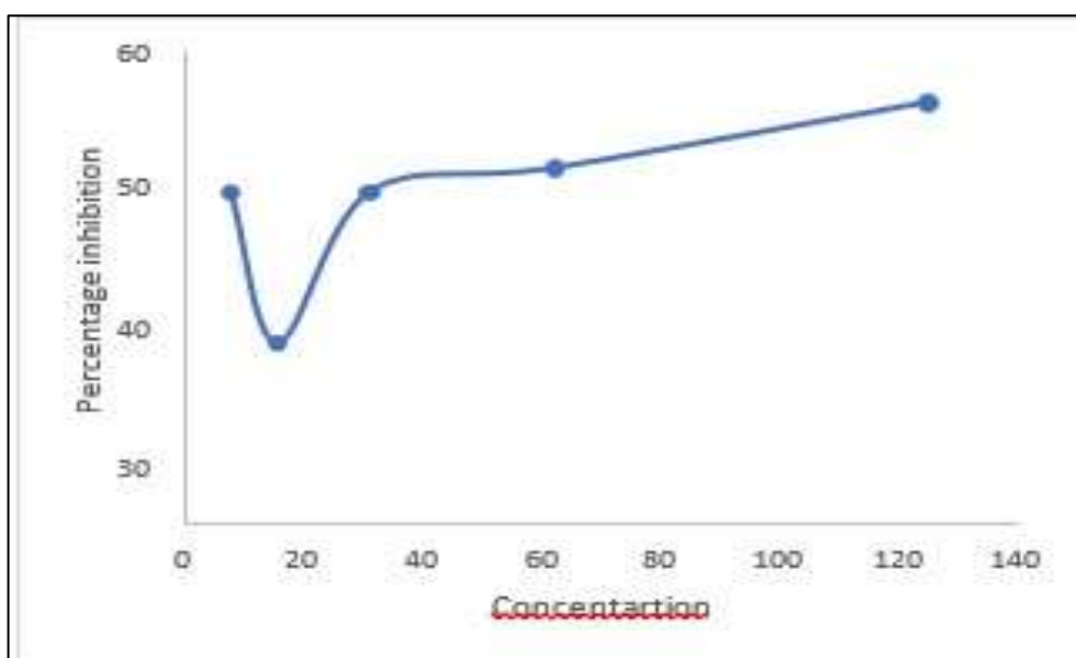
Graph 13: Graph represents anti biofilm activity of Bacillus subtilis
