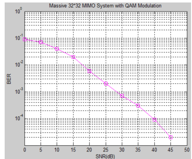
Figure 7: BER vs SNR for Matched Filter Detection Spectrum Sensing 32 \times 32 System
