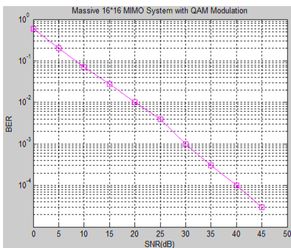
Figure 6: BER vs SNR for Matched Filter Detection Spectrum Sensing 16 \times 16 System
