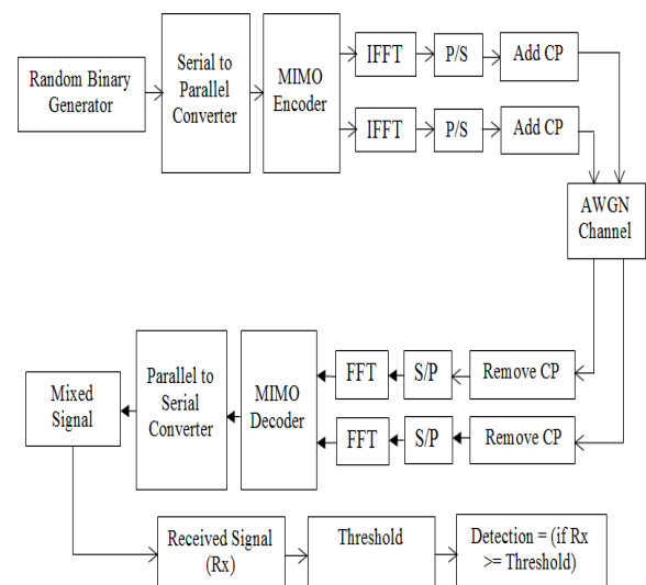
Figure 4: Design of MIMO-OFDM System using Matched Filter Spectrum Sensing Cognitive Radio Network
